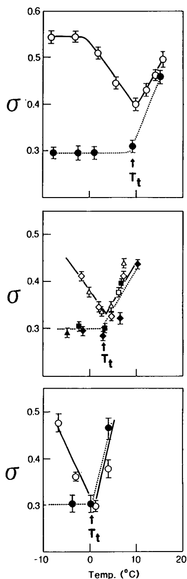
FIGURE 6 Temperature-dependence of spectral saturation. Spectral saturation ( \sigma ) for native SR (open symbols) and vesicles made from extracted SR lipids (solid symbols) as a function of temperature for the following stearic acid spin labels. (Top) 5-SASL; (middle) 7-SASL (diamonds), 10-SASL (squares), 12-SASL (triangles); (bottom) 16-SASL. T_t is the threshold temperature below which spectral saturation is minimal for stearic acid spin labels in extracted lipid.
