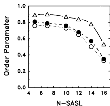
FIGURE 5 Apparent order parameter profile. Solid circles represent measurements of stearic acid spin labels in extracted SR lipids at -4^\circ\text{C} , used to model the bulk lipids in native SR membranes at 0^\circ\text{C} (Fig. 4, second row, dotted lines). Open triangles represent the restricted spectral component obtained subsequent to the spectral subtraction of the bulk lipid component (Fig. 4, third row). Open circles correspond to extracted SR lipids at 0^\circ\text{C} . N-SASL refers to the position of the nitroxide spin label relative to the \alpha -carbon of the stearic acid. Order parameters are calculated from the observed spectral anisotropy subsequent to spectral deconvolution using Eqs. 1 and 2 (see Methods).
