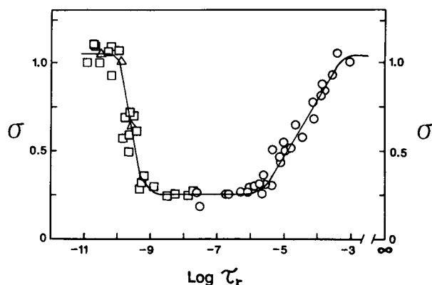
FIGURE 3 Sensitivity of ST-EPR to isotropic rotational motion. The rotational correlation time of the isotropic model systems MSL-Hb in glycerol/water solutions (circles) or TANOL in either glycerol/water (squares) or sec-butyl-benzene (triangles) solutions were determined with Eq. 4. Spectral saturation ( \sigma ) is defined in Eq. 6. The rotational correlation time was altered by varying either the glycerol concentration and the temperature (circles, squares) or by varying the temperature only (triangles).
